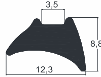
AYKİM02 CAM FITİLİ Glass Gasket
