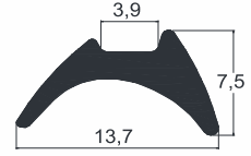
BM11 C60 FITİLİ C60 Gasket
