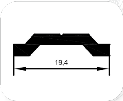
Polyamid Tij
