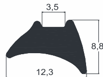
Glass Gasket
